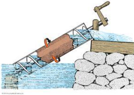
Archimedes screw
